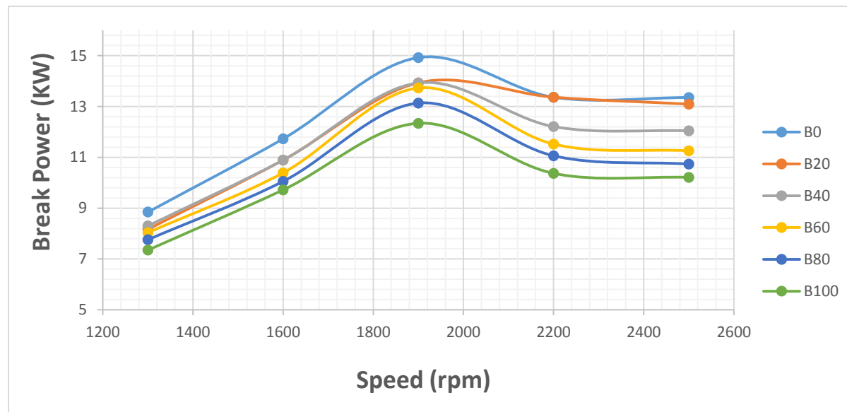
Figure 3.4: Break power with Engine Speed for Standard Diesel and Biodiesel Blends from D.edulis.
