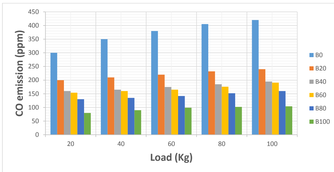
Figure 3.5: Variation of CO Emission with Load for standard diesel, Biodiesel from D.edulis and Blends at 1900 rpm.
